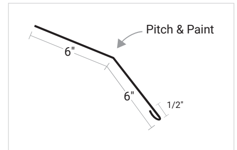
Pbr Upper Transition
