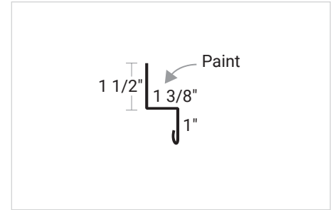
PBR Z-Flashing
