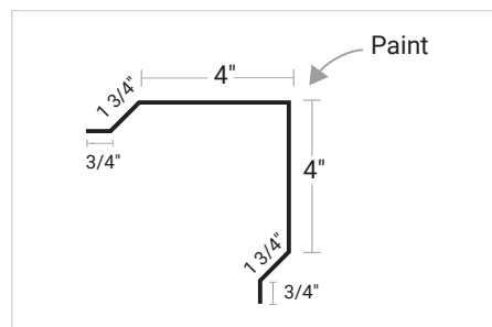
PBR Outside Corner
