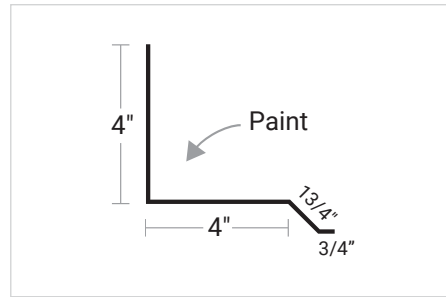
PBR Sidewall
