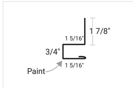
PBR Square Base Trim
