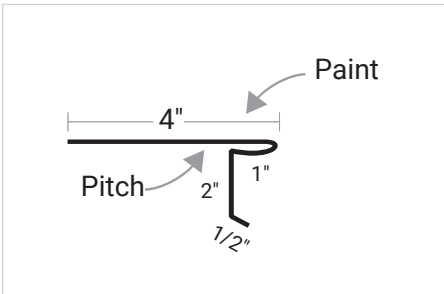
Style D Eave
