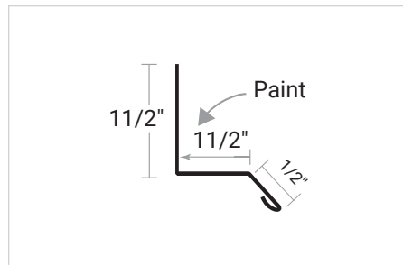
PBR 1 1/2" Window Drip Cap
