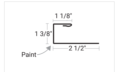
PBR J-Metal
