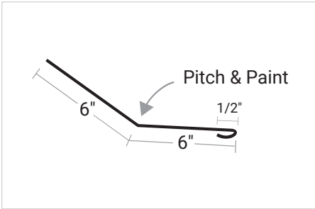
Lower Transition
