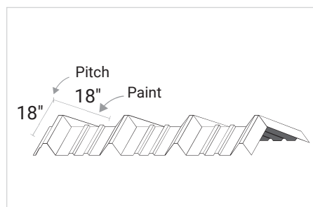
Profile - Ridge
