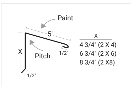
PBR Front Cap (High Eave)
