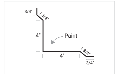
PBR Inside Corner
