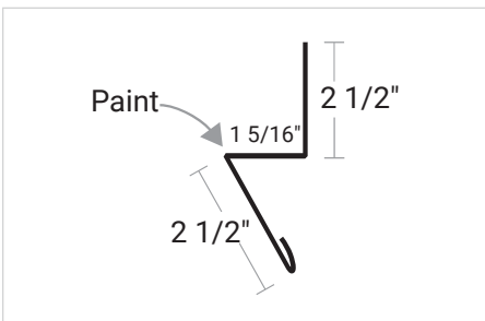
PBR Z-Base Trim
