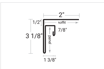
PBR F+J 1 1/4" x 1/2" (Panel to Soffit)
