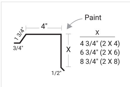
PBR Gable/Rake
