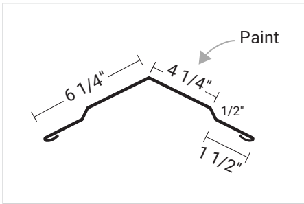
Rollformed Ridge Cap
