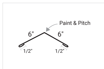
Hip Ridge
