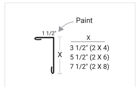
Door Post Trim
