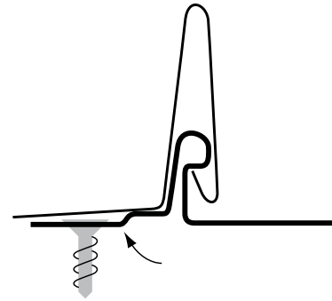
Fastening Clip is Rollformed into the panel
